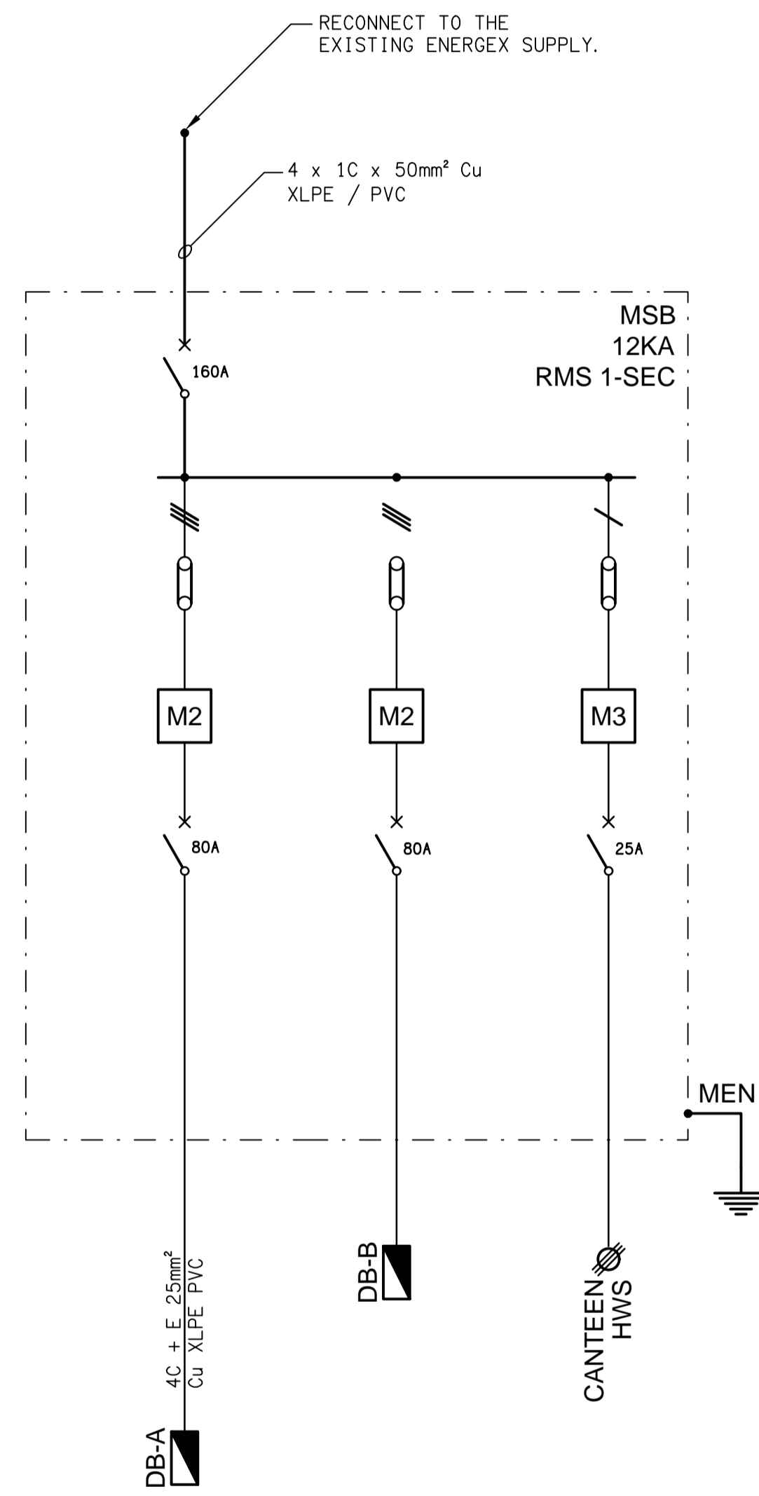
SCHEMATIC MSB-A CONFIGURATION NOT TO SCALE
